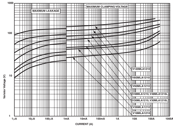
FIGURE 9. LIMIT V-I CHARACTERISTIC FOR V18MLA1210 TO V120MLA1210
