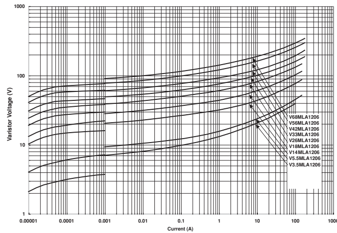
FIGURE 6. LIMIT V-I CHARACTERISTIC FOR V3.5MLA1206 TO V68MLA1206
