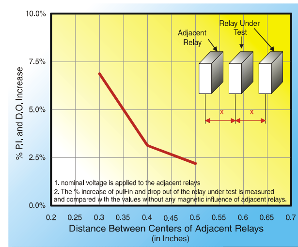
Figure 3. EMR Spacing Requirements
