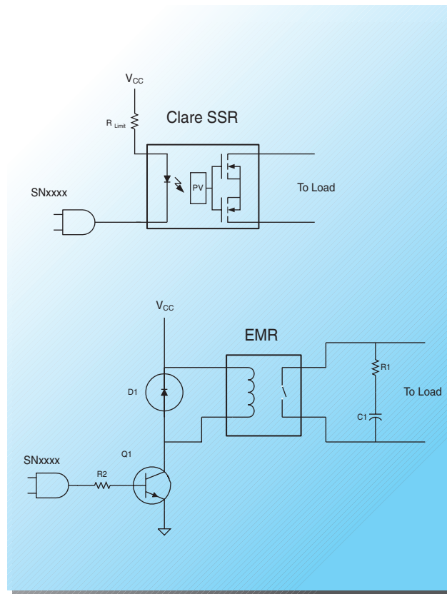
Figure 6. SSR and EMR Drive Circuit Comparison
