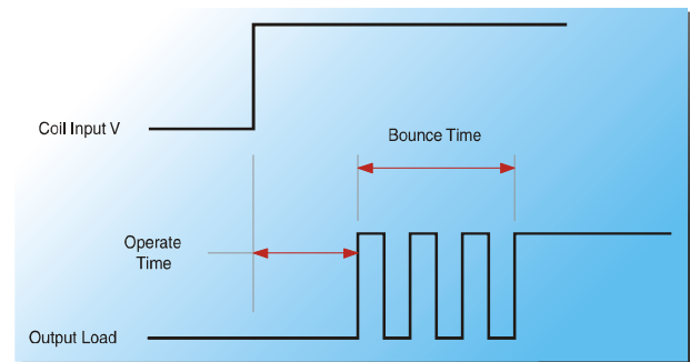
Figure 4. EMR Contact Bounce
