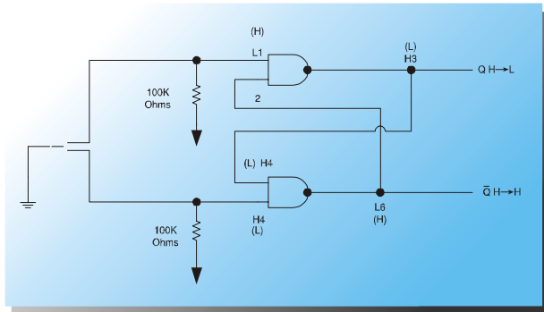
Figure 5. Contact Bounce Circuit
