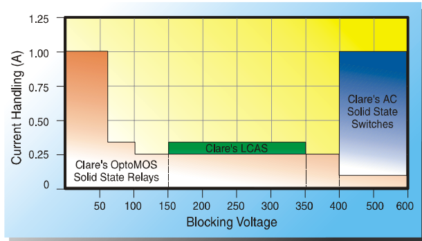
Figure 1. Clare Solid-State Relays
