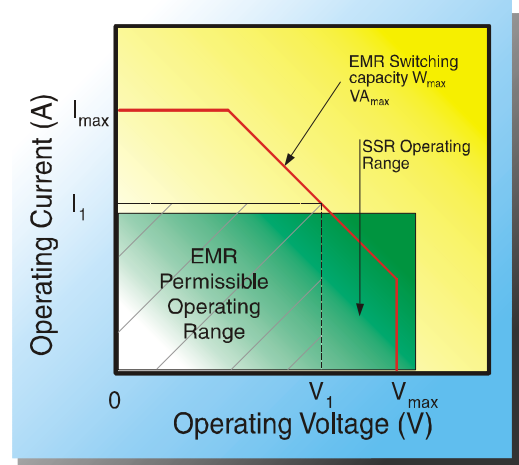
Figure 2. Relay Derating Curves
