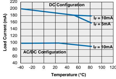
PLA193 Typical Load Current vs. Temperature
