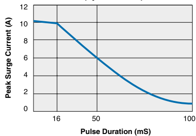
CPC1965Y Maximum Surge Current (non-repetitive) ( T_J = 50^\circ\text{C} max)
