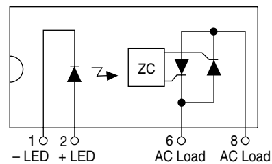
CPC1965Y Pinout
