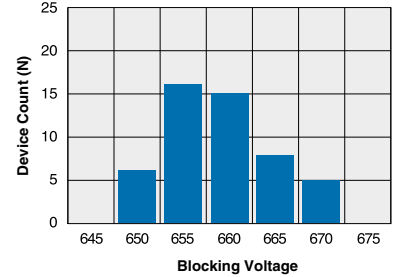
CPC1965Y Typical Blocking Voltage Distribution (Ambient Temperature = 25°C)
