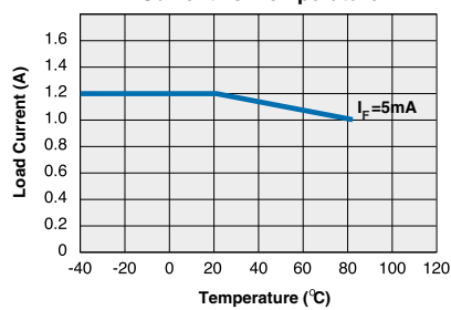
CPC1965Y Typical Maximum Load Current vs. Temperature
