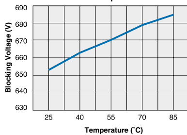
CPC1965Y Typical Blocking Voltage vs. Temperature
