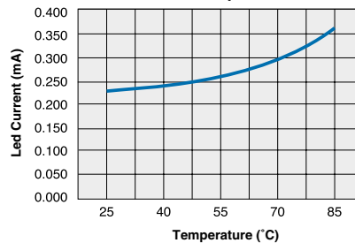
CPC1965Y Typical I_F for Switch Operation Over Temperature
