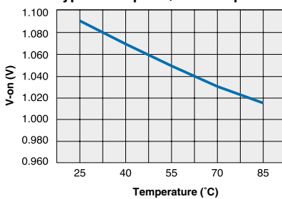
CPC1965Y Typical Output V_F vs. Temperature
