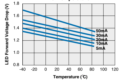
CPC1965Y Typical LED Forward Voltage Drop vs. Temperature
